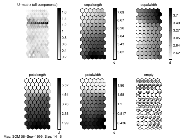
Figure 5: Visualization of the SOM of Iris data. U-matrix on top left, then component planes, and map unit labels on bottom right. The six figures are linked by position: in each figure, the hexagon in a certain position corresponds to the same map unit. In the U-matrix, additional hexagons exist between all pairs of neighboring map units. For example, the map unit in top left corner has low values for sepal length, petal length and width, and relatively high value for sepal width. The label associated with the map unit is 'se' (Setosa) and from the U-matrix it can be seen that the unit is very close to its neighbors.
