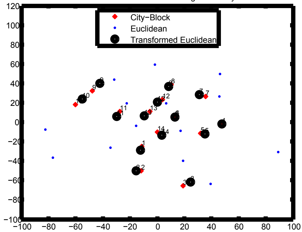
Procrustean Transformation of the Euclidean Scaling to the City-Block Coordinates
